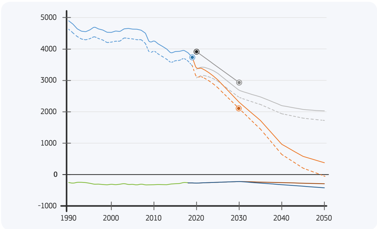
Figure 1 Total EU 27 GHG emissions (including international aviation) and removals 1990-2019, current 2030 Target and proposed step-up, projected emissions 2020 – 2050 with existing ('baseline') and with additional measures necessary to achieve climate neutrality ('net zero') by 2050 vi
