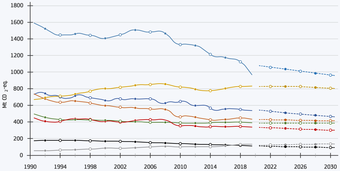
Figure 1 EU-27 GHG emissions by sector, historical data (1990-2019) and projections (2020-2030) 9
